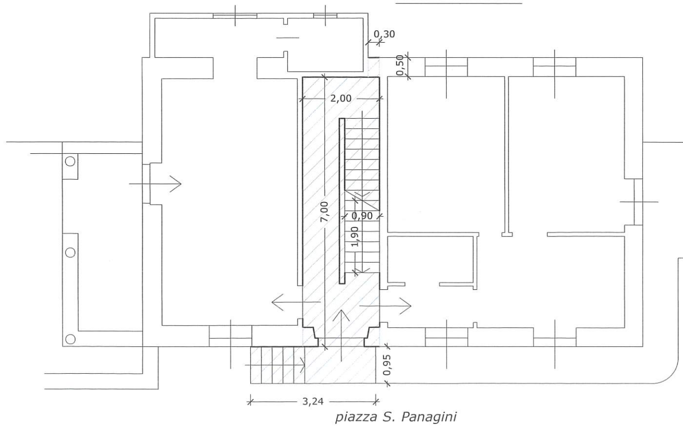
PIANO TERRENO
